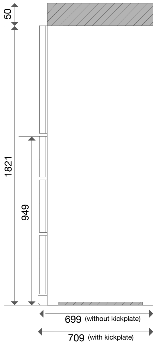
Side View
