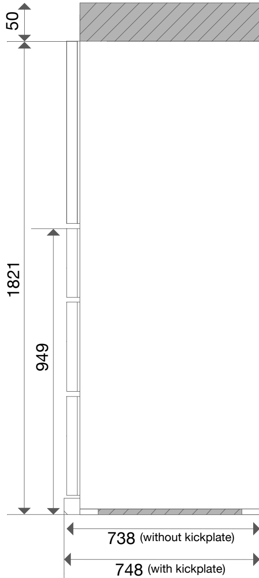
Side View
